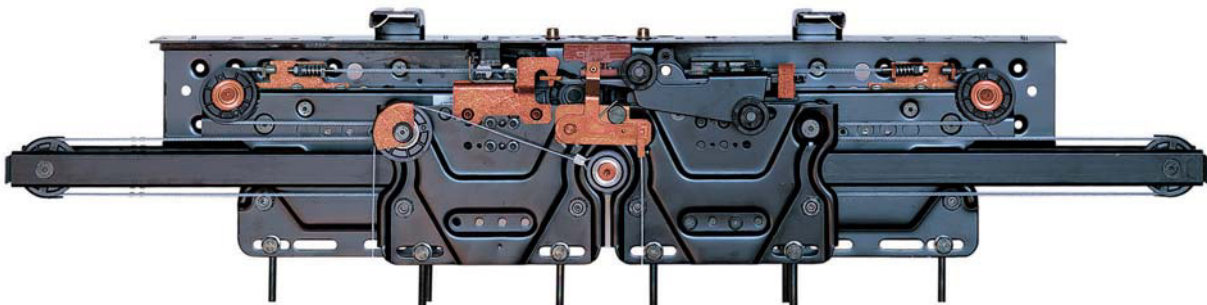
Schachtmechanismus Mod. HYDRA TYP 43/R. Landing mechanism mod. Hydra type 43/R.
